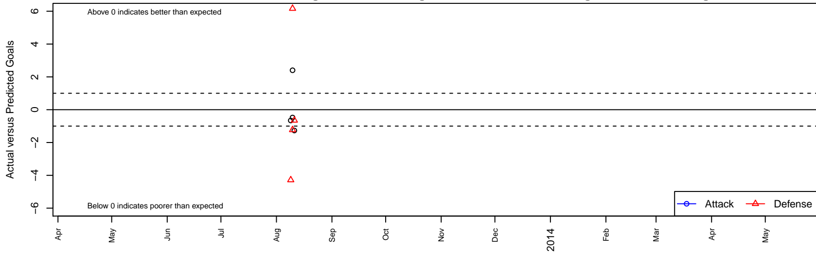
FC EI Tri B97 Dots are actual minus expected GF (blue circles) and GA (red triangles). Blue line is smoothed change in attack strength. Red is smoothed change in defense strength.
